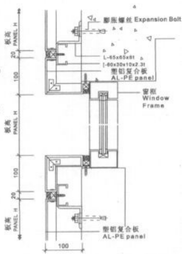
开窗接板立断面 VERTICAL WALL TO WINDOW INSTALLATION DETAIL
