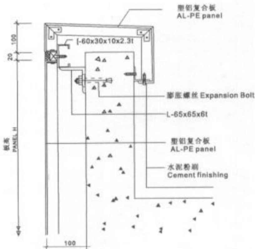
女儿墙立面图 PARAPET WALL VERTICAL CAPPING SECTION
